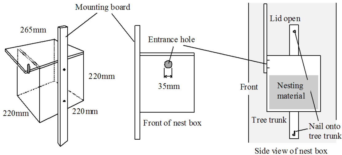
Figure 2 Example of nest box design and specifications.
